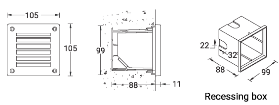
Recessing box
