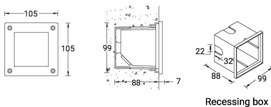
Recessing box
