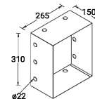
Recessing box
