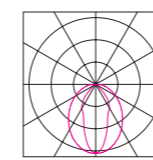
TITAN LED 45°
