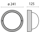
EKO+ 21 LED 21
